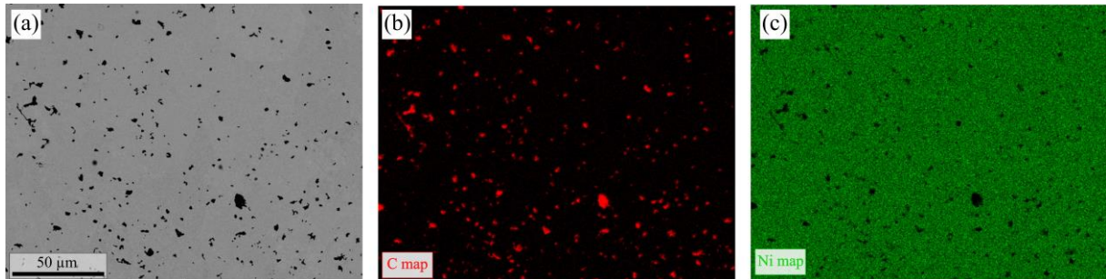
Figure 2 – (a) Secondary electron micrograph of the surface of the sample treated at 1300 °C. (b) EDS chemical map of the C distribution (in red) and (c) Ni distribution (in green).
